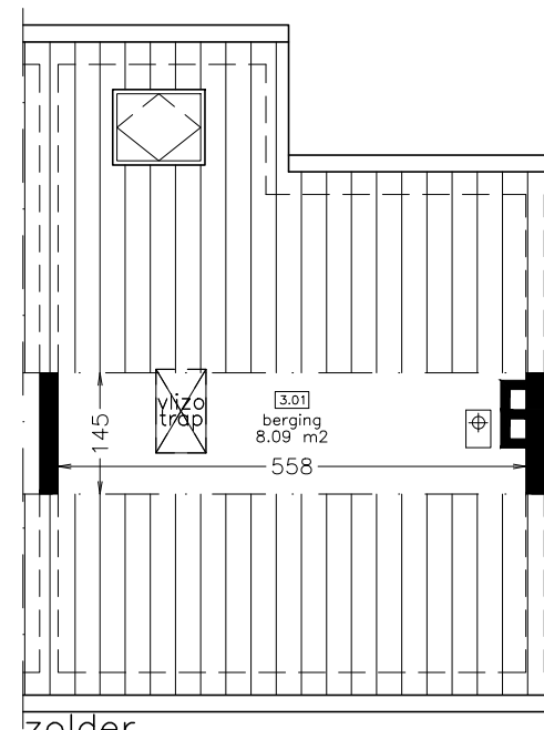
zolder
